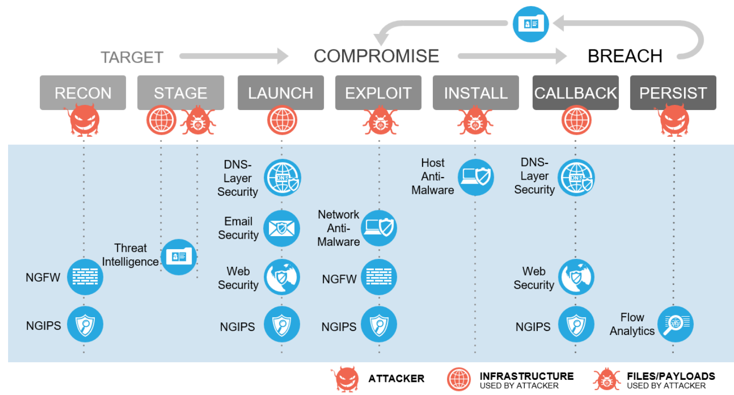
Figure 6—Breaking the Kill Chain with Security Capabilities
