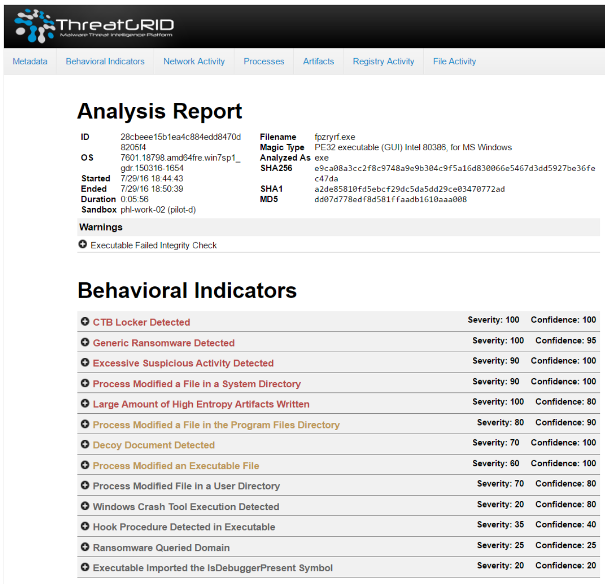
Figure 14—File Analysis Report
