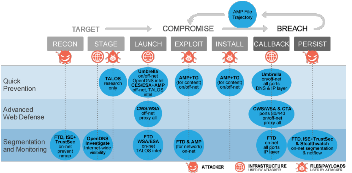
Figure 16—Products Replace Capabilities in the Kill Chain
